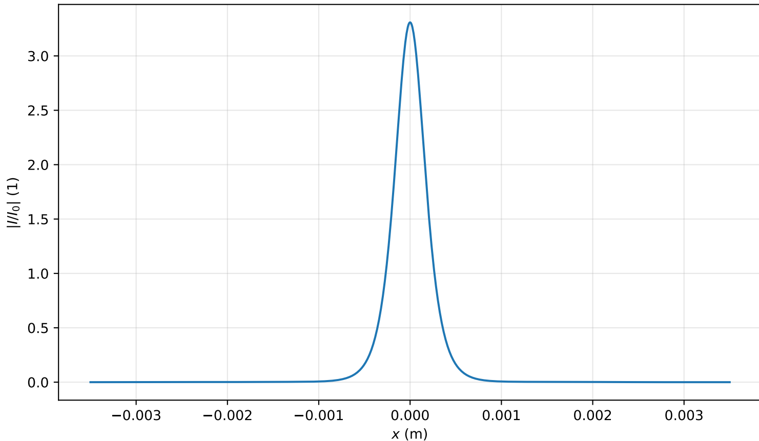
Intensity profile I(x, y = 0, z = 3.901m)/I_0 , P_{in}=1.0P_{cr} , artificial time
